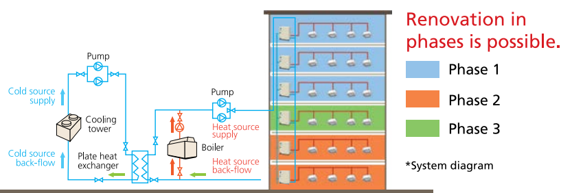
Water cooled VRV IV W series
